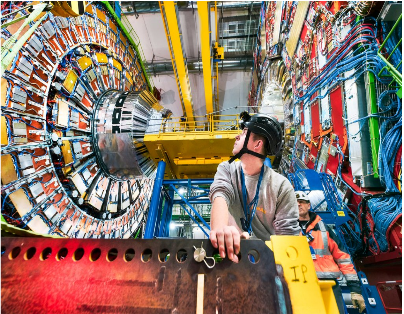
Workers prepared the Large Hadron Collider at CERN in Switzerland for a shutdown period spanning two years in 2019. Credit...Maximilien Brice and Julien Marius Ordan/CERN, via Science Source
